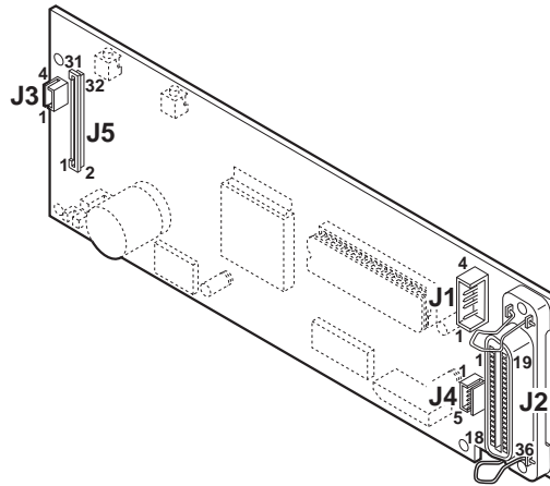
Figure 5-3 Logic Board
