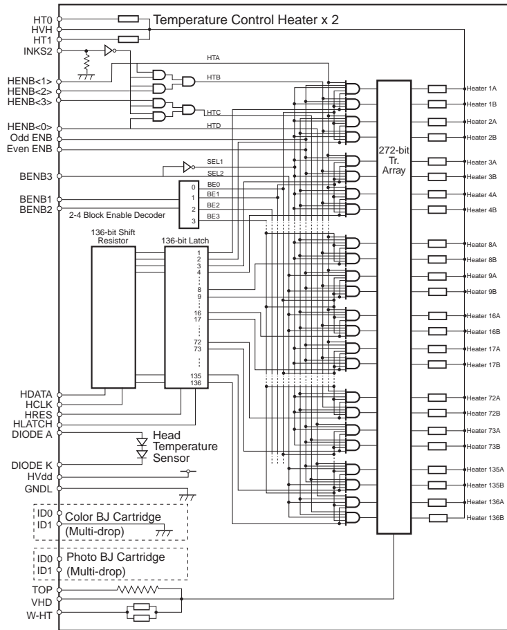
Color BJ cartridge (Multi-Drop) and photo BJ cartridge (Multi-Drop) have the same circuit configuration except for the ID1 connection.
